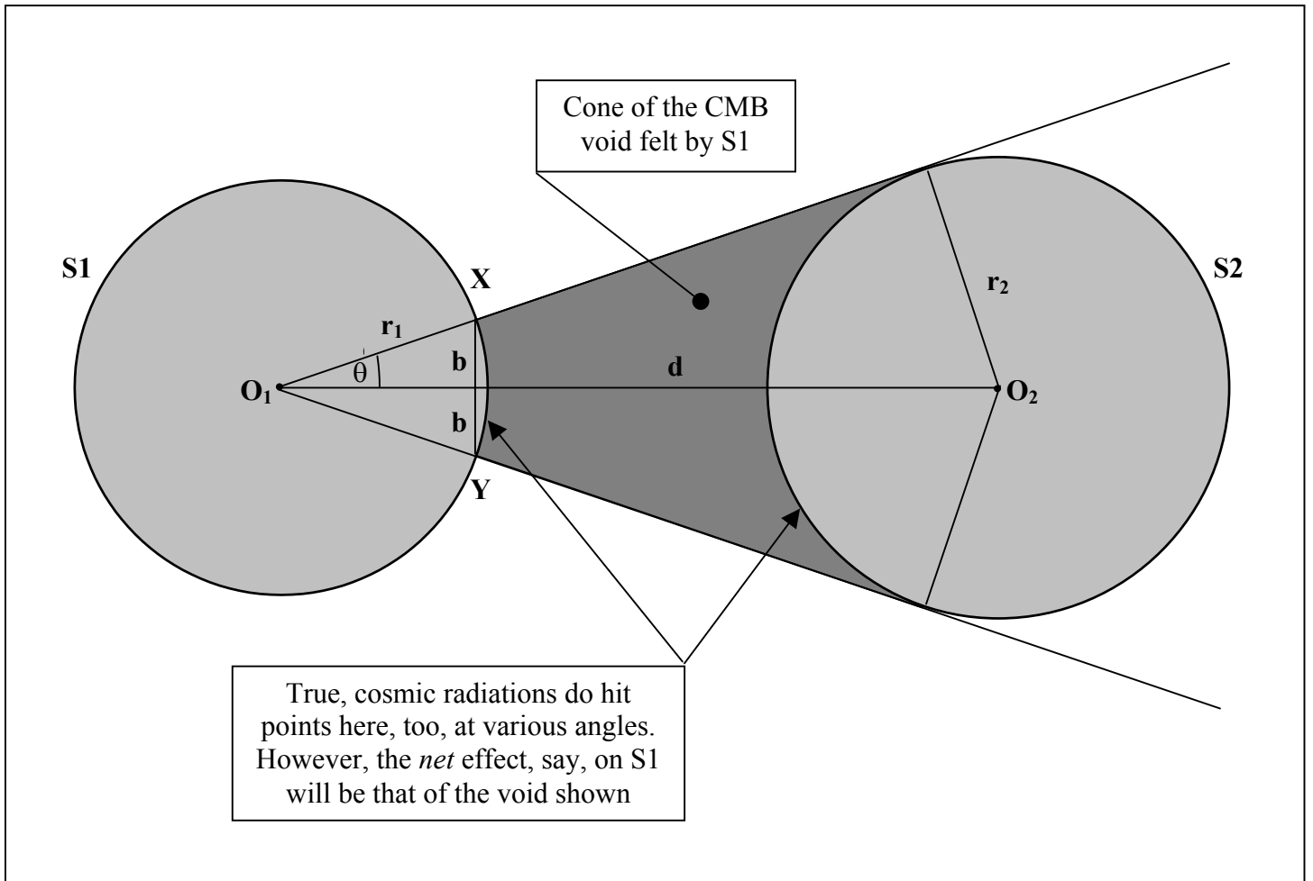
Figure 1. The CMB shielding of S1 by S2. Only the analytically equivalent gravitational spheres, S1 and S2, of the two celestial bodies are shown here.
