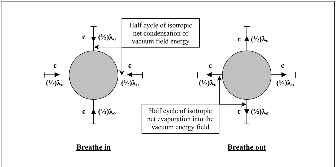
Figure 2. Body at rest. The exchanges between body and the outside vacuum energy field are the same all around. Velocity c and wavelength \lambda_0 are with respect to absolute space, the space of the CMB, in which the body is at rest.
