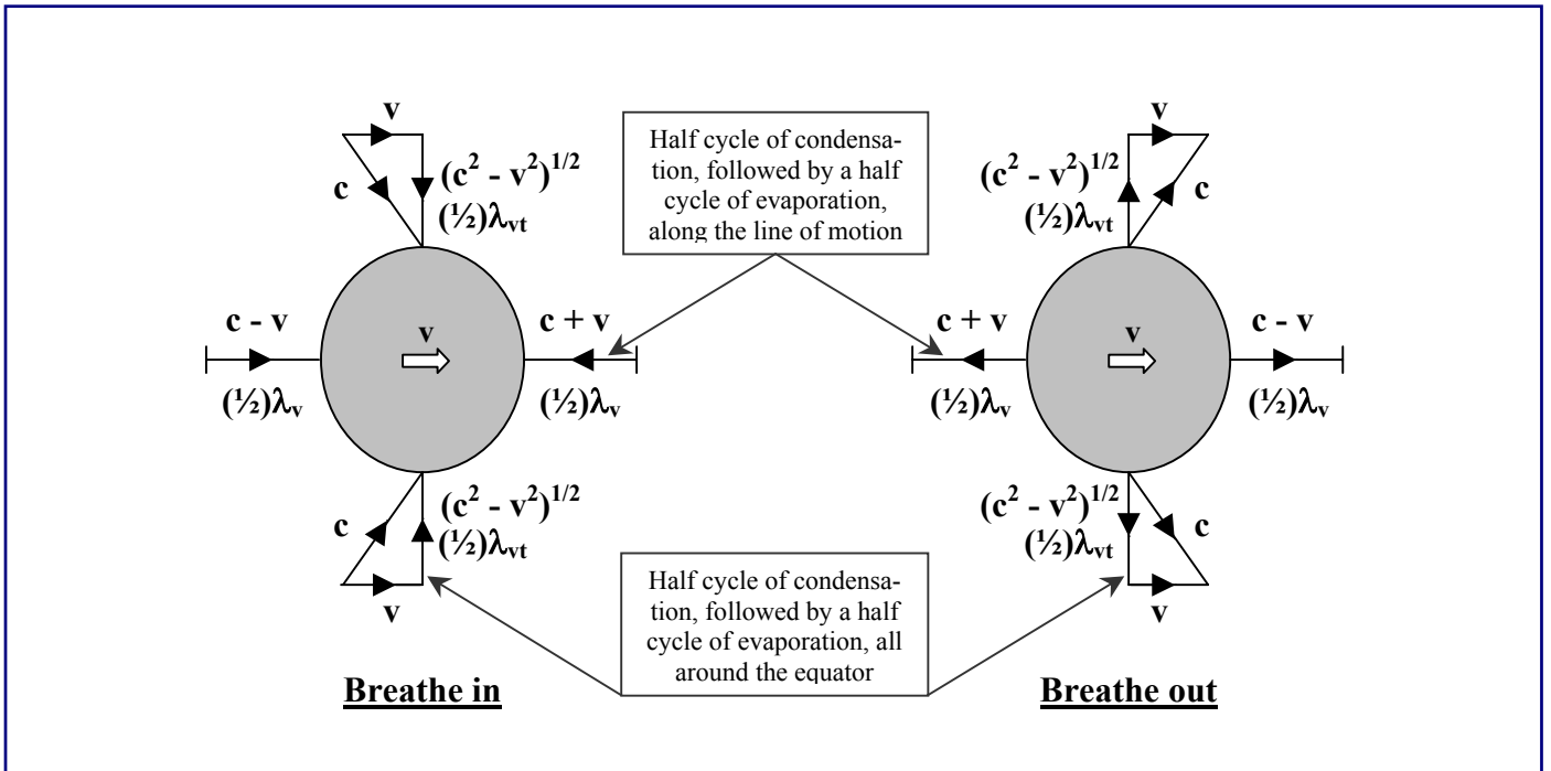
Figure 3. Body at velocity v . And the exchanges become polar. Individual velocities c and v are with respect to absolute space, the space of the CMB; wavelengths and combined velocities are relative to body moving at v .
